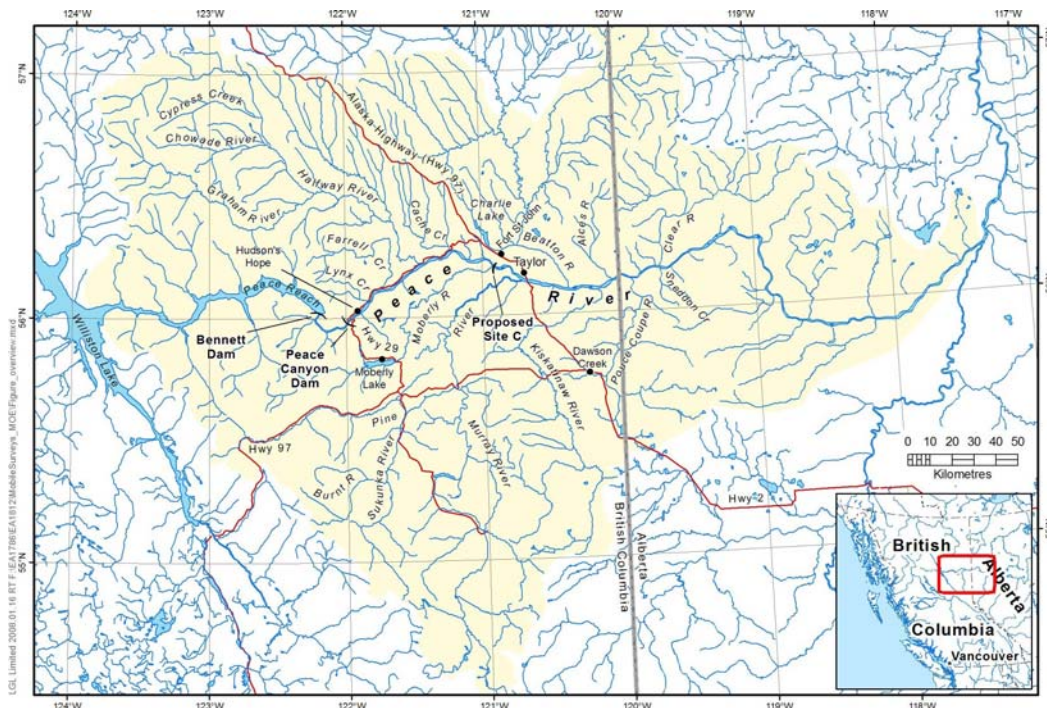
Figure 1: Existing and potential hydroelectric development on the Peace River in northeast British Columbia
