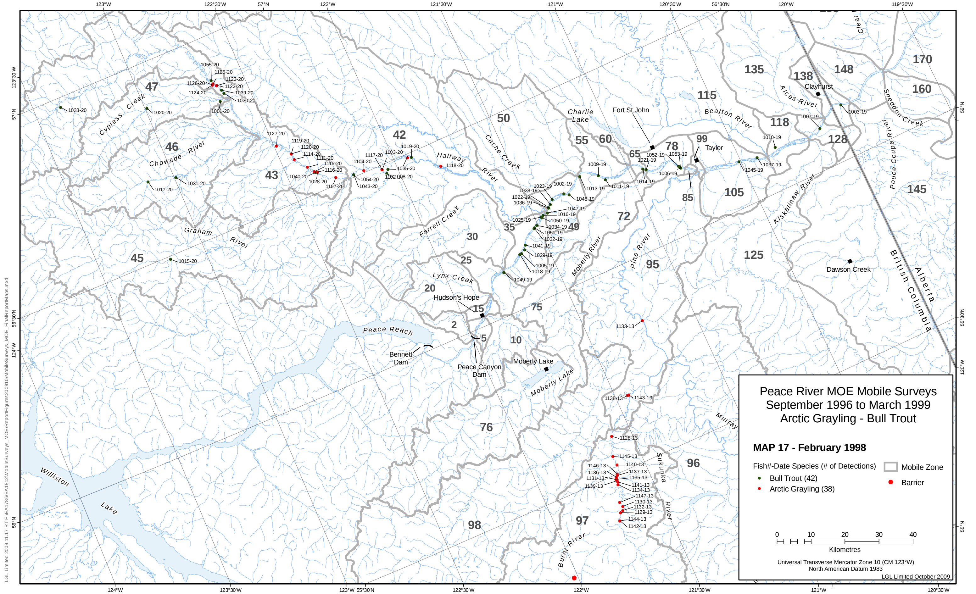
Map 17: Mobile survey detections for February 1998
