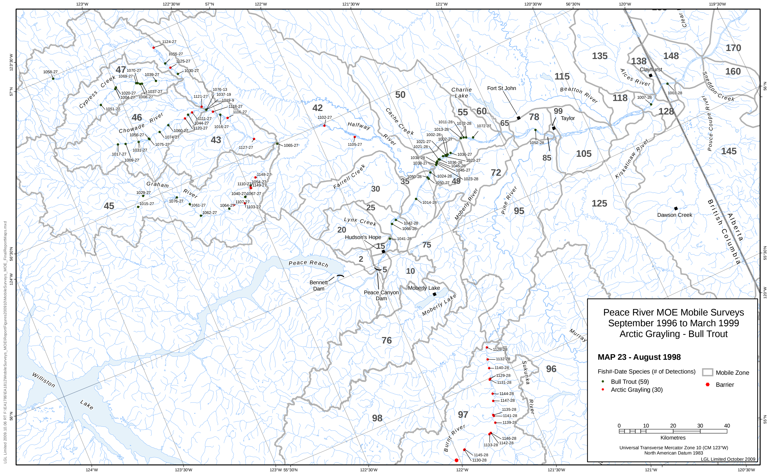
Map 23: Mobile survey detections for August 1998
