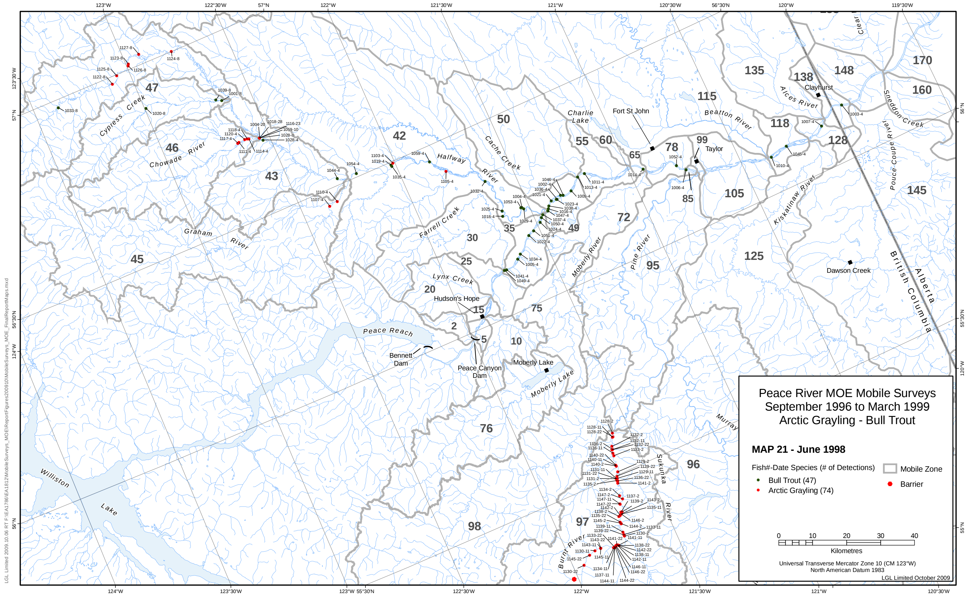
Map 21: Mobile survey detections for June 1998
