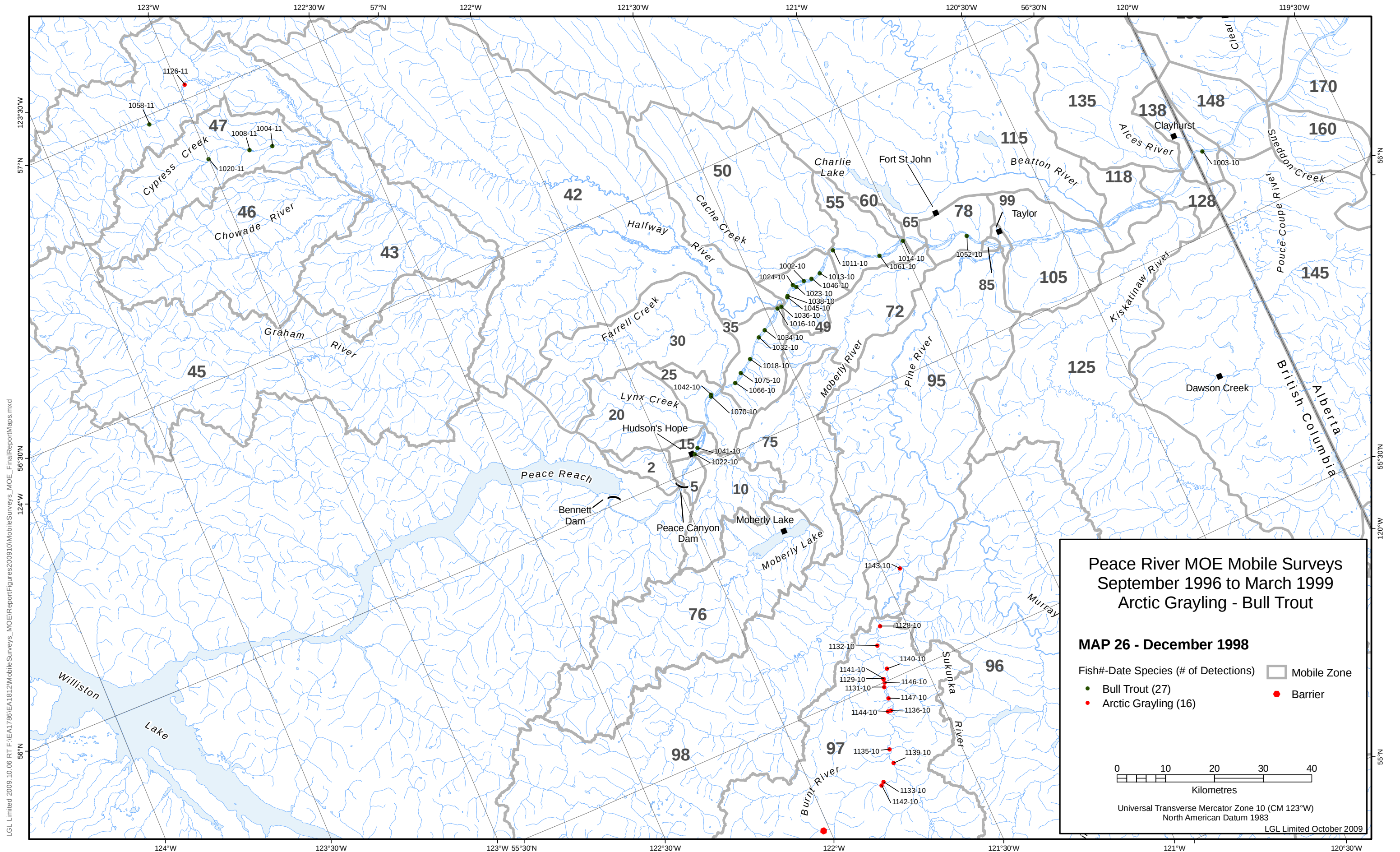
Map 26: Mobile survey detections for December 1998
