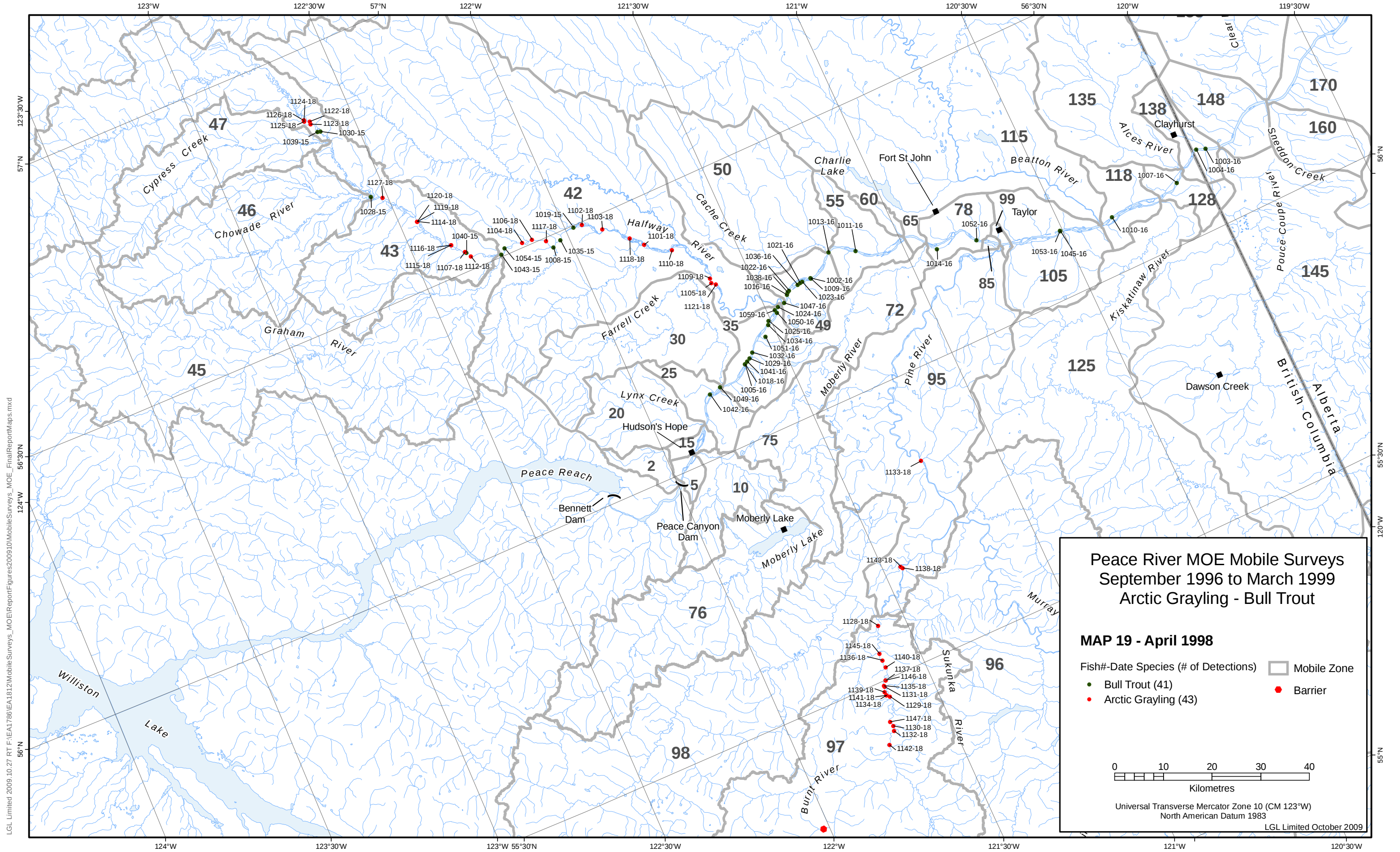
Map 19: Mobile survey detections for April 1998
