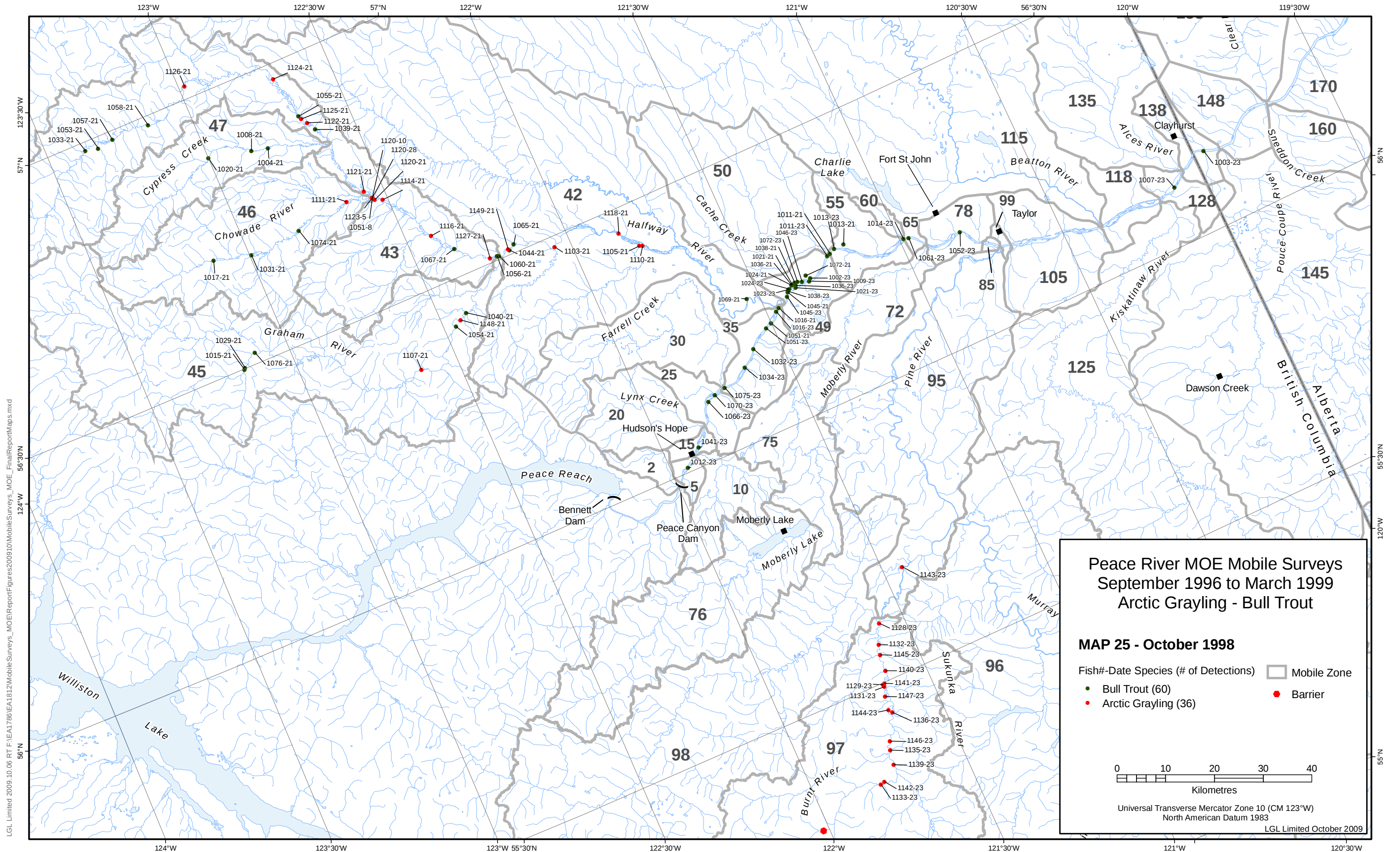
Map 25: Mobile survey detections for October 1998
