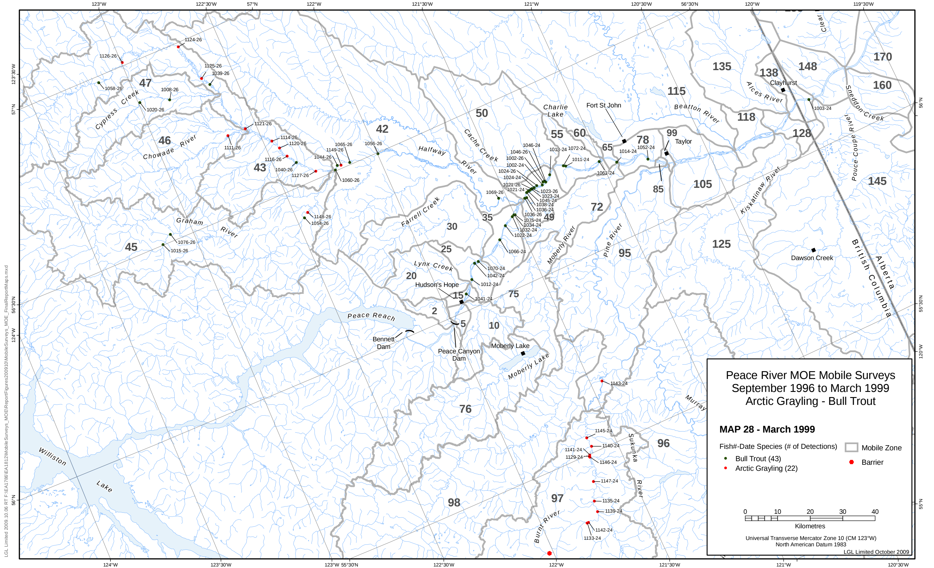
Map 28: Mobile survey detections for March 1999
