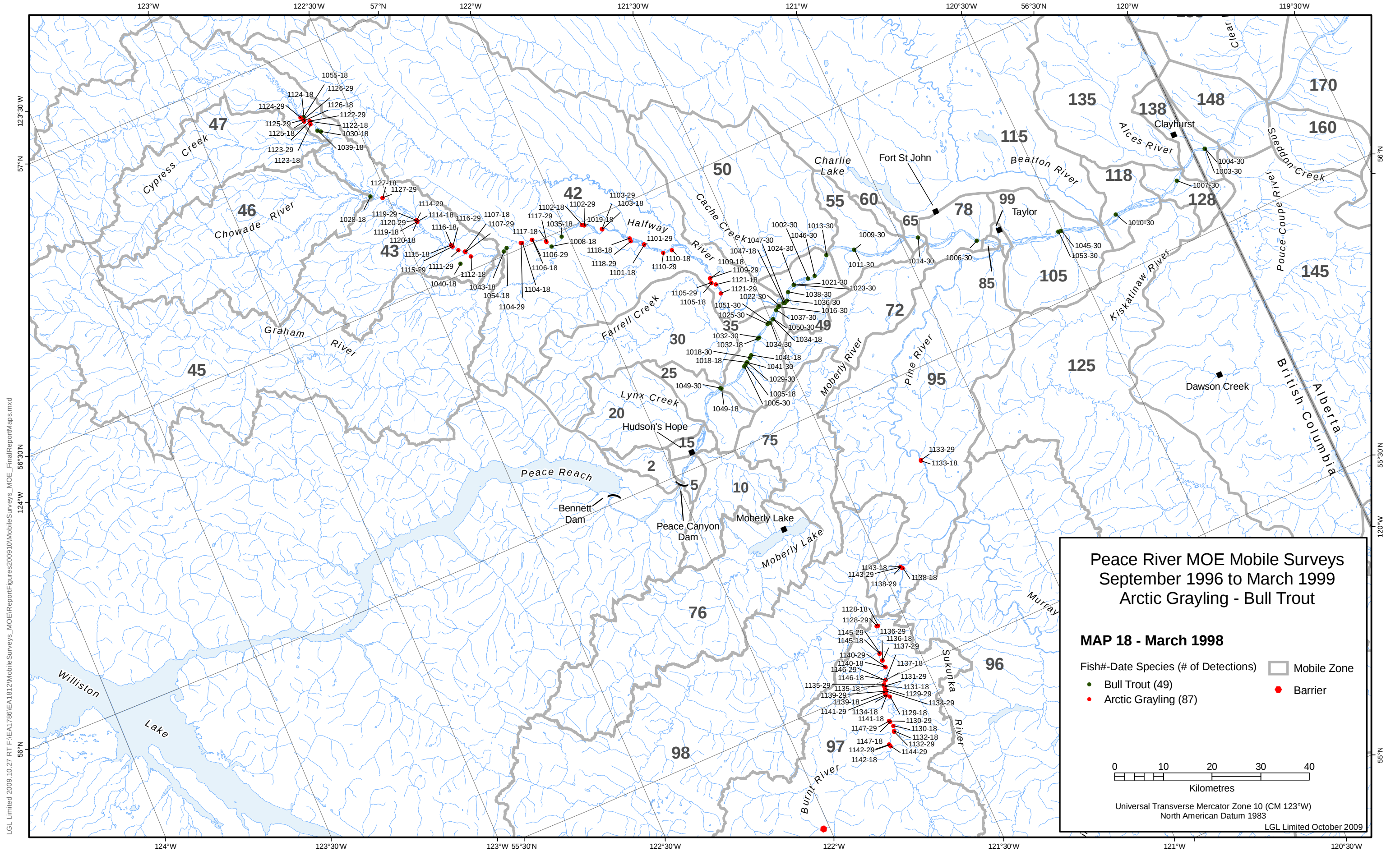
Map 18: Mobile survey detections for March 1998
