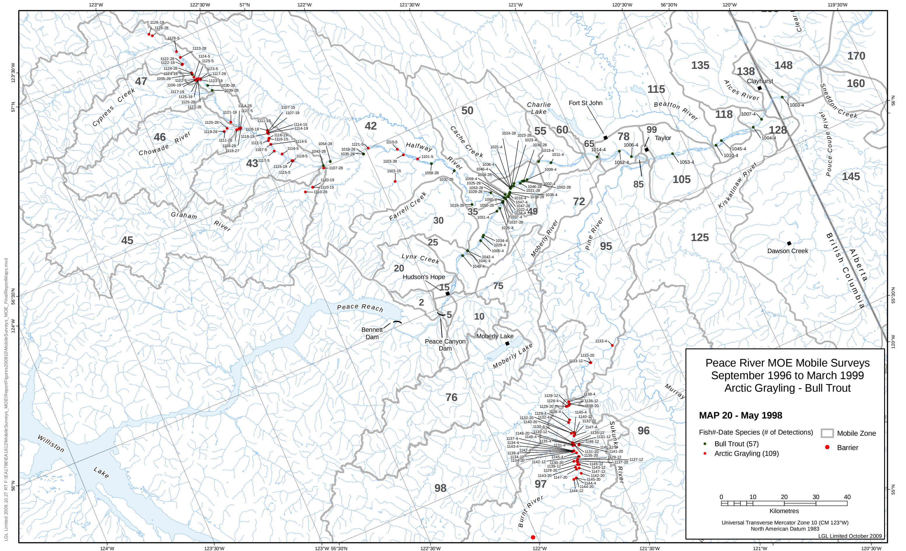
Map 20: Mobile survey detections for May 1998
