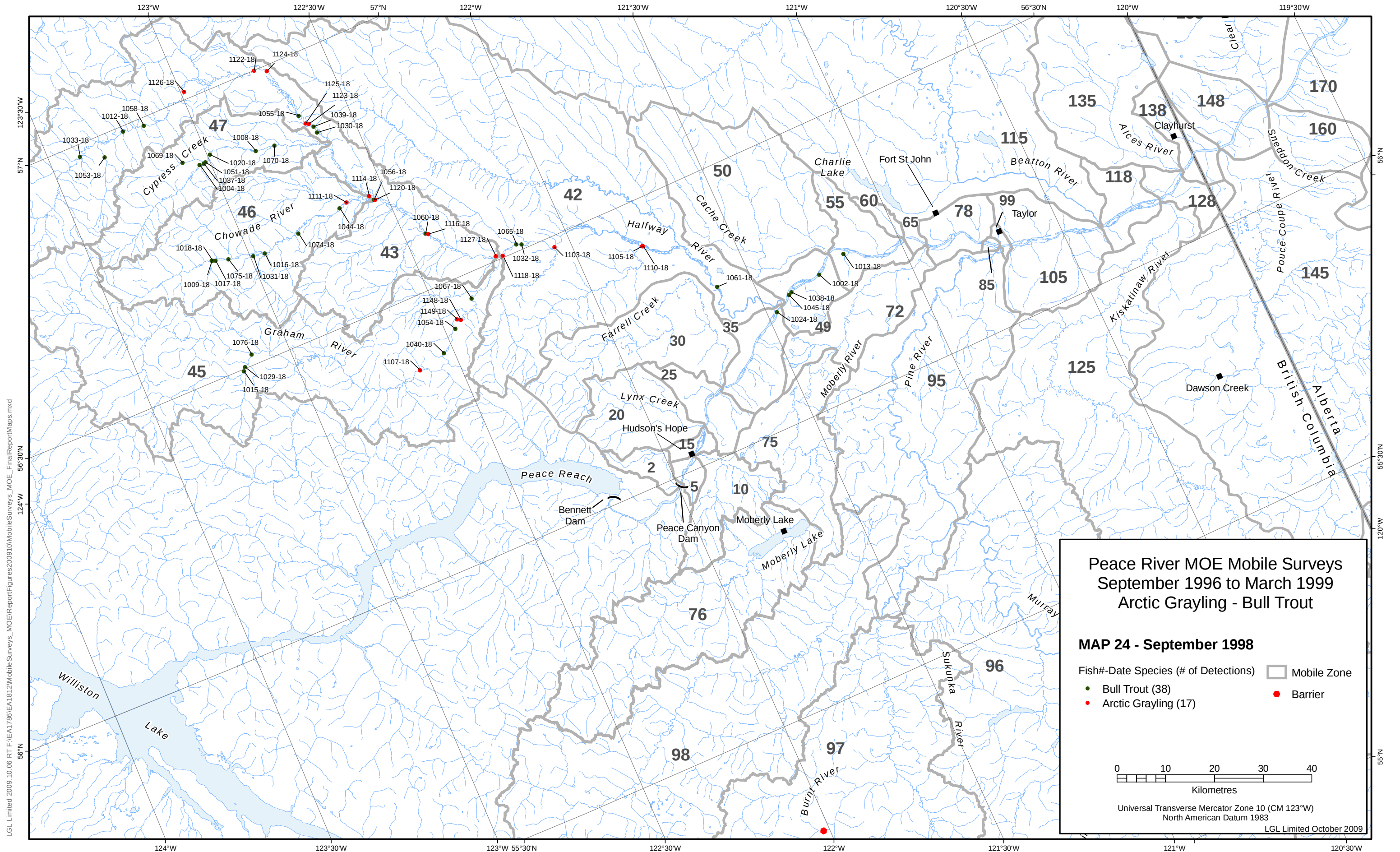
Map 24: Mobile survey detections for September 1998
